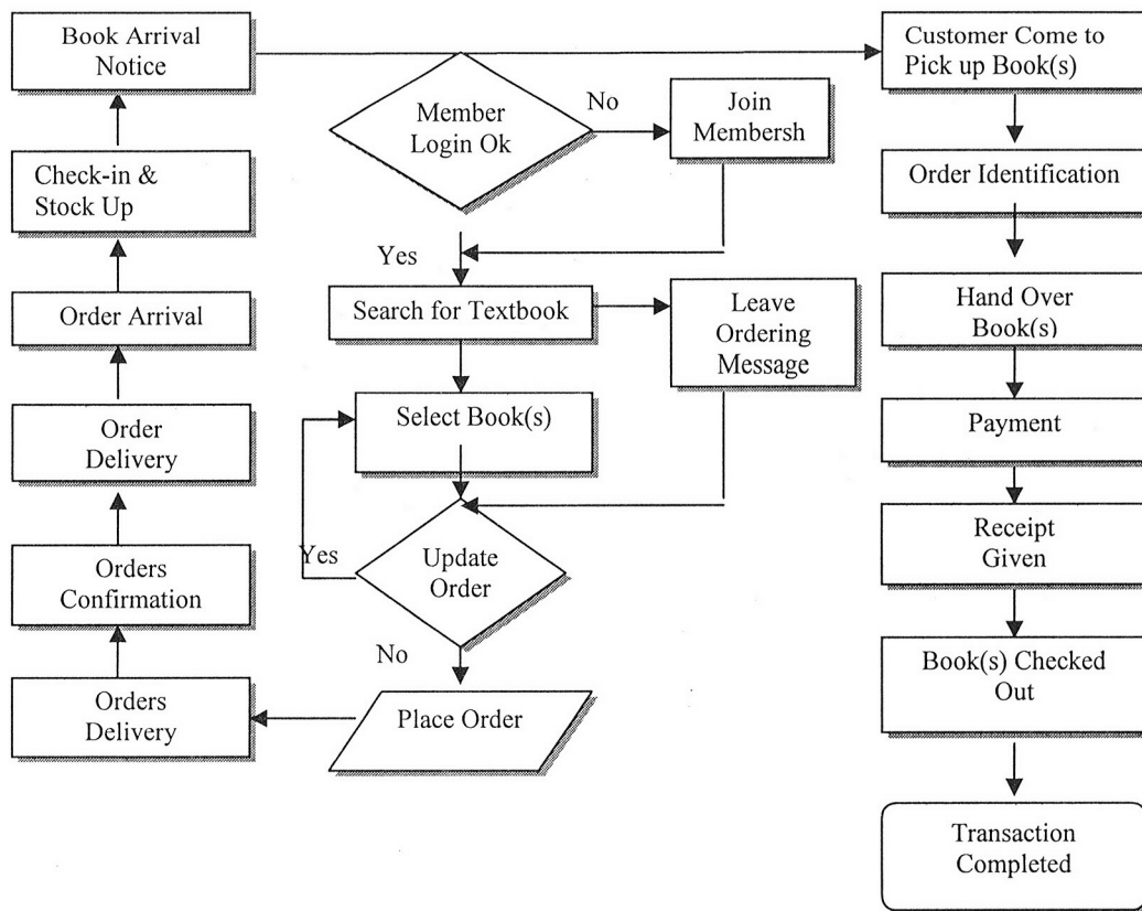
Figure 4 - Transactional Flow
